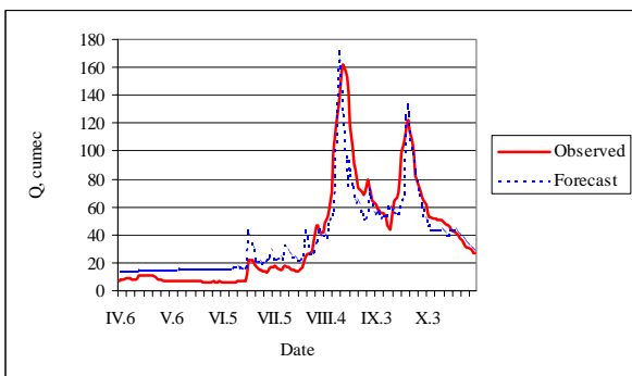
Figure 3. Forecasted and observed hydrograph, Kherlen-Baganuur-Underkhaan
