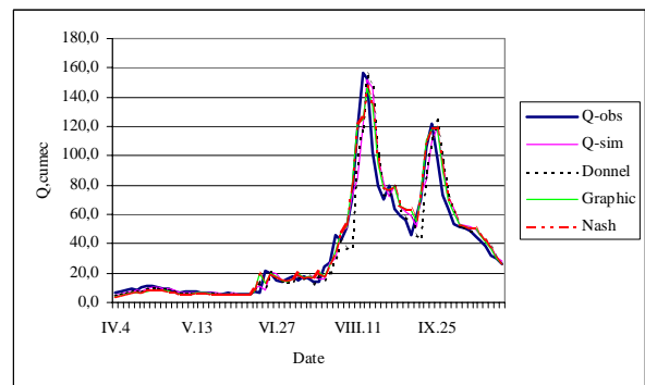
Figure 4. Simulated hydrograph along the Kherlen river
