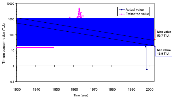
Fig.9 Residence time of Groundwater in Type A area estimated from time series variation of tritium concentration in precipitation
