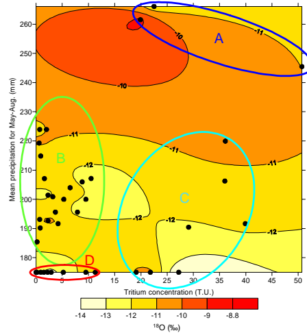
Fig.6 Distribution of 18 O ratio in groundwater on the relation figure of tritium concentration and precipitation.
