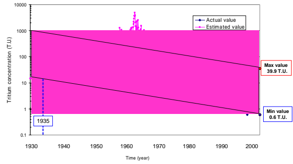
Fig.11 Residence time of Groundwater in Type B-C and C-D areas estimated from time series variation of tritium concentration in precipitation
