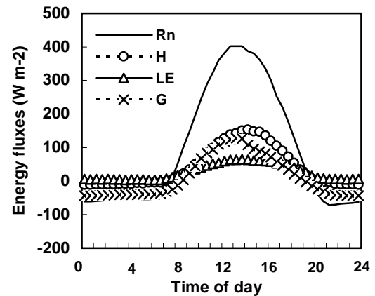
Fig. 3. Diurnal trends of energy fluxes.
