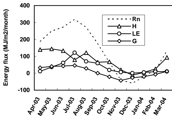
Fig. 4. Annual variation in energy fluxes.
