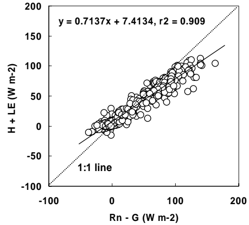
Fig. 2 Energy balance check.
